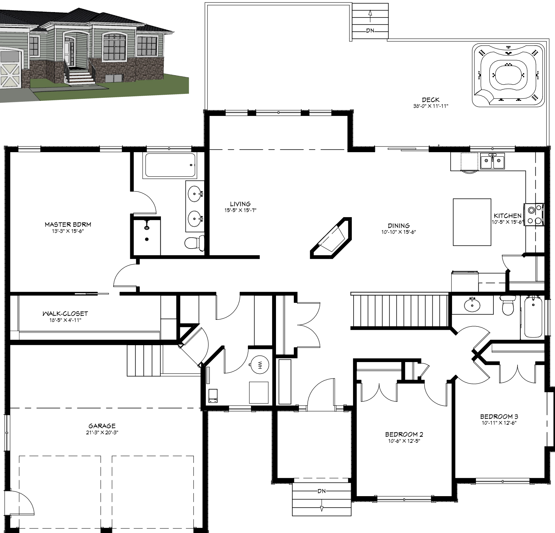
MAIN FLOOR PLAN: 1855 SQ.FT.
