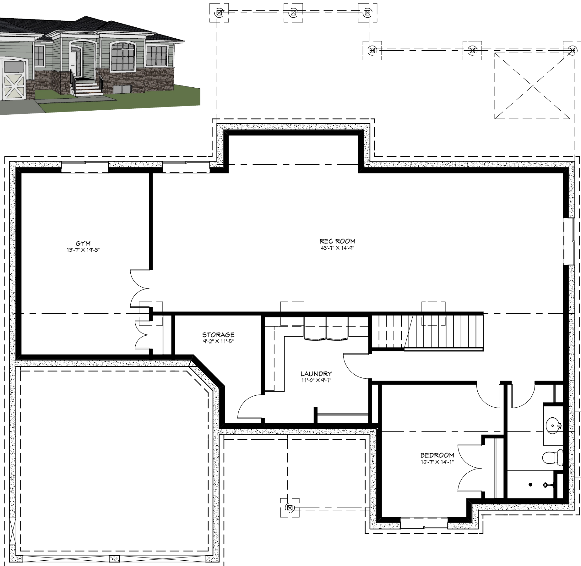
BASEMENT PLAN: 1714 SQ.FT.
