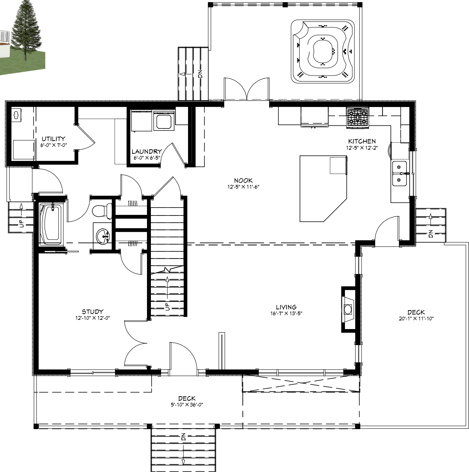
MAIN FLOOR PLAN: 1195 SQ.FT.
